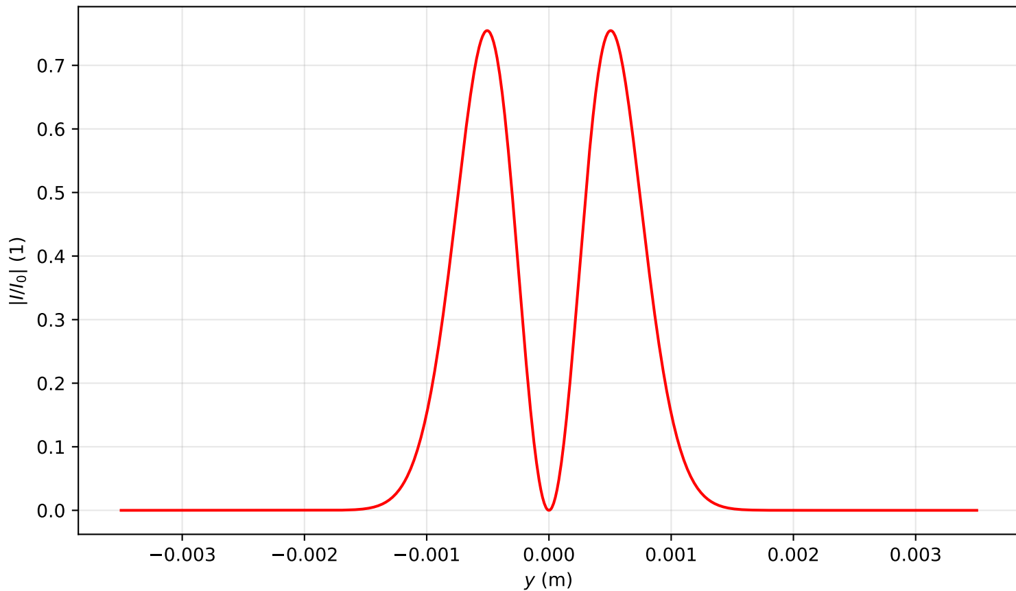
Intensity profile I(x=0, y, z=0.398)/I_0 , \text{Pin}=0.5\text{Pcr} , artificial time
